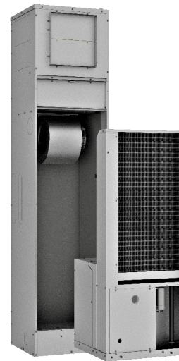
SLIDE IN HRCX CHASSIS TO HR CABINET
