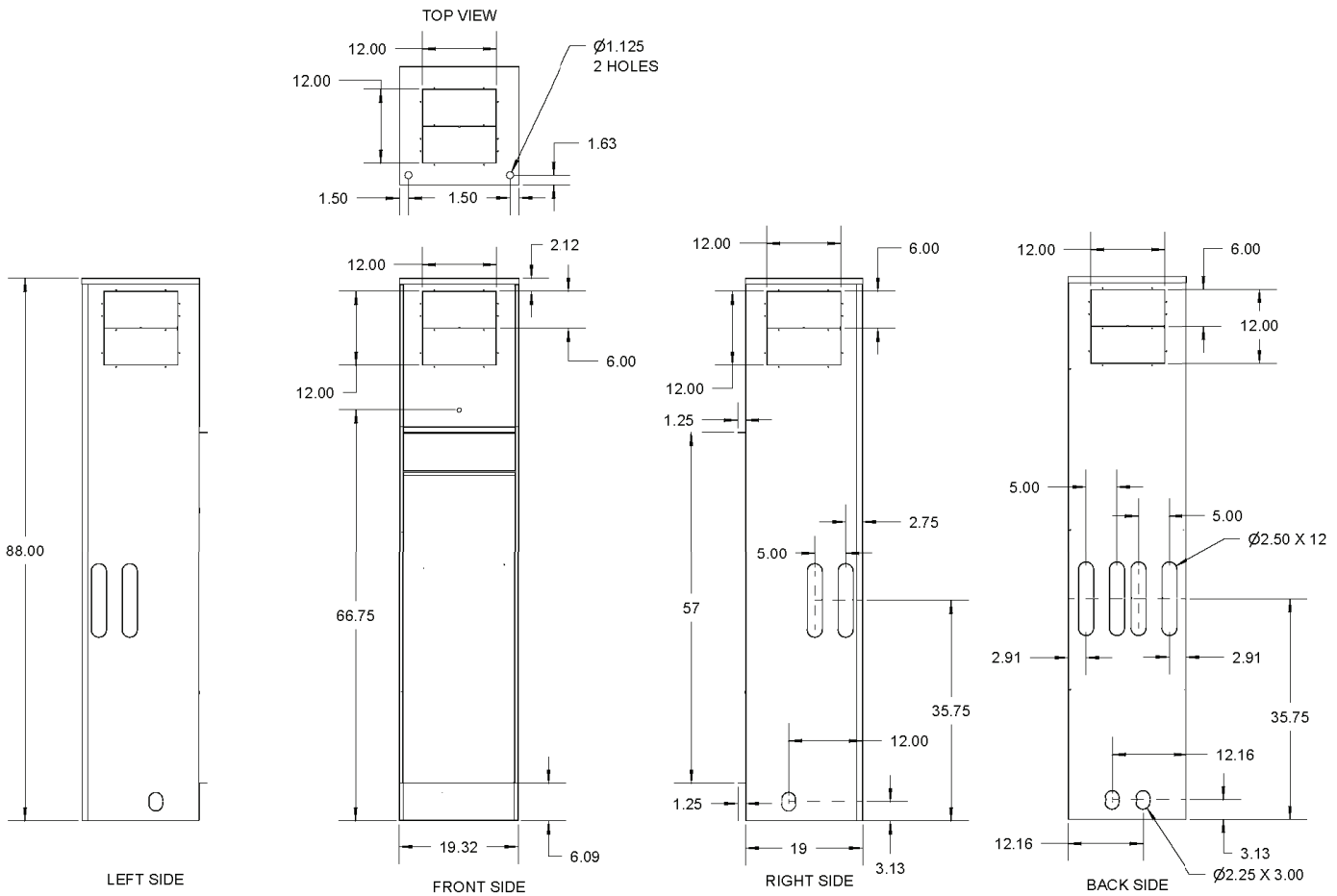
HT Vertical High Rise Heat Pump Cabinet
