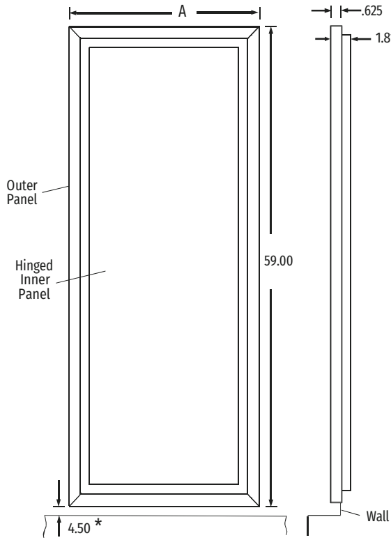
Front View Standard Panel
