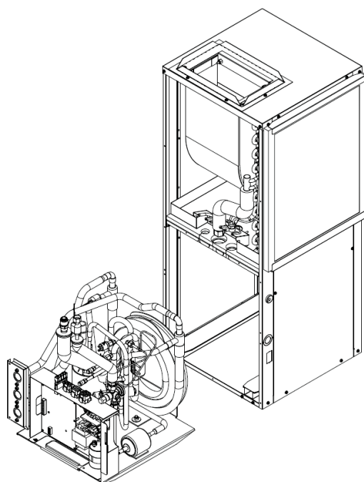
Slide out refrigeration section
